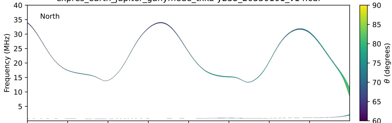
expres_earth_jupiter_ganymede_txka-y235_20330101_v14.cdf
