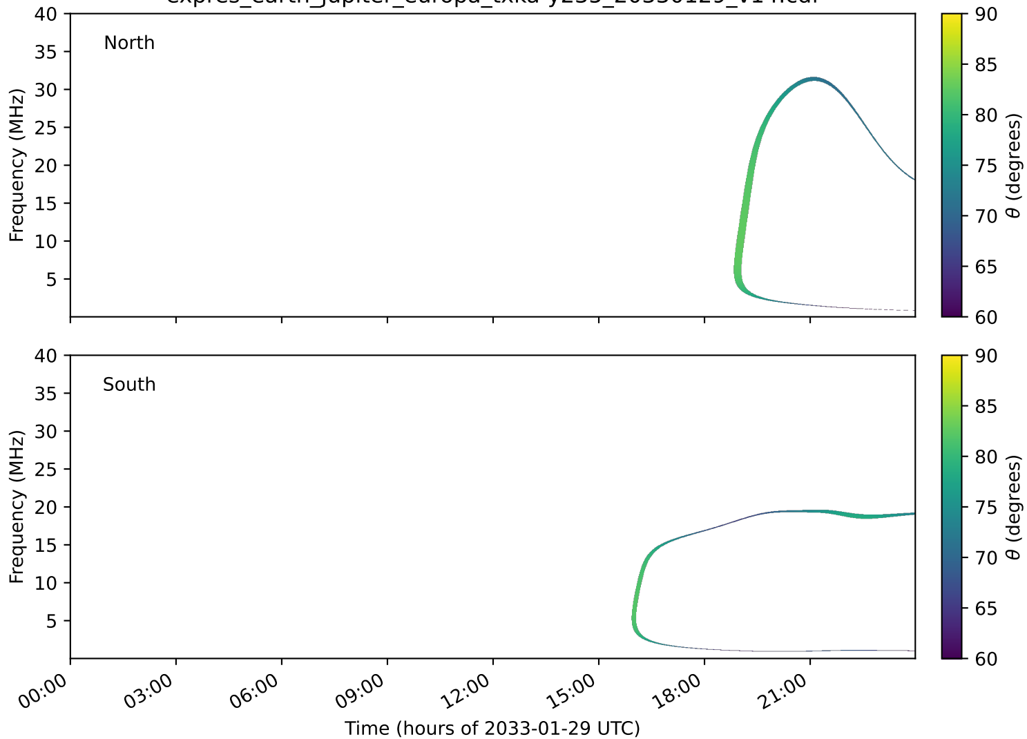
expres_earth_jupiter_europa_txka-y235_20330129_v14.cdf
