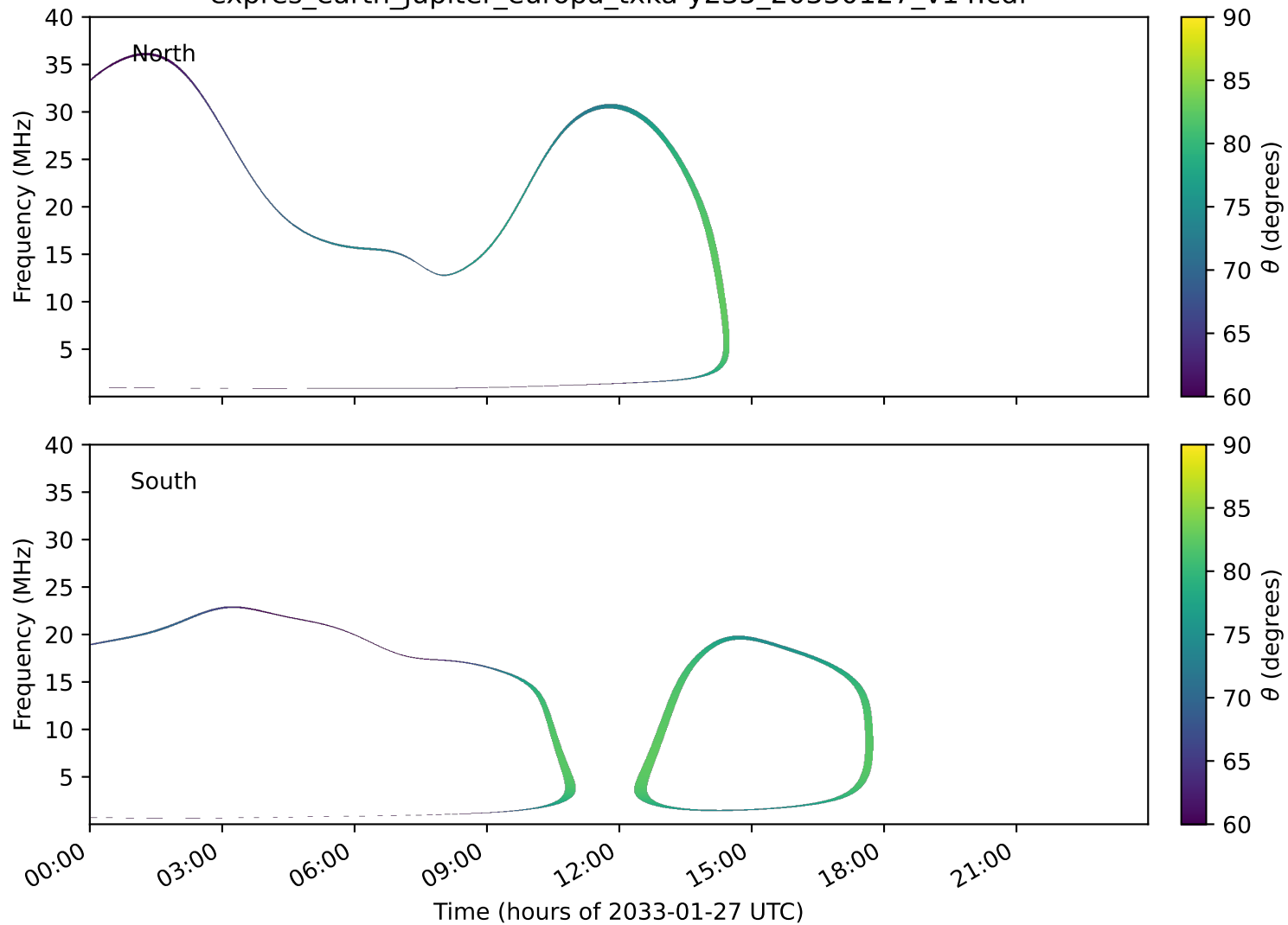
expres_earth_jupiter_europa_txka-y235_20330127_v14.cdf
