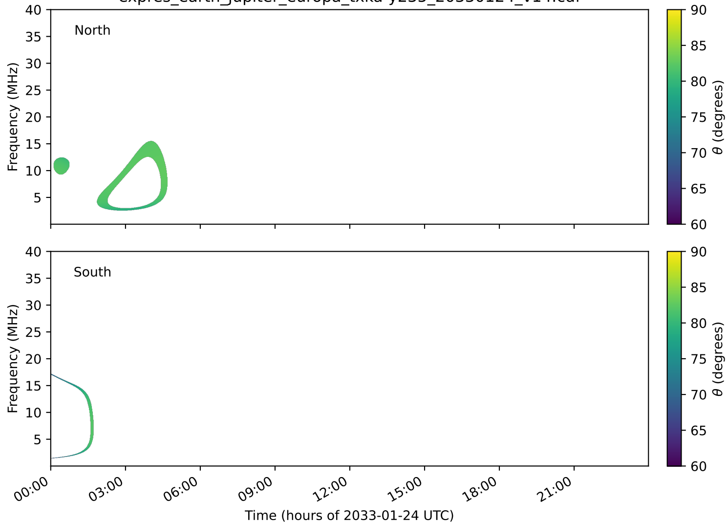
expres_earth_jupiter_europa_txka-y235_20330124_v14.cdf
