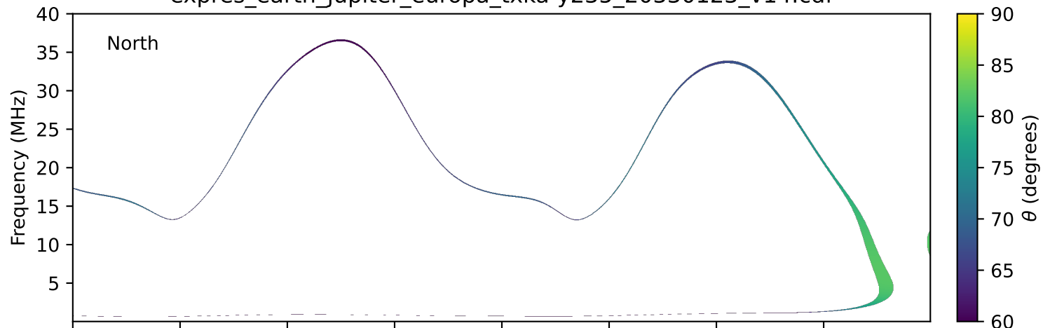
expres_earth_jupiter_europa_txka-y235_20330123_v14.cdf
