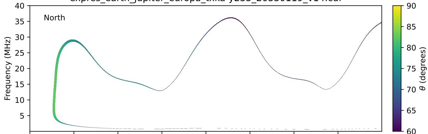
expres_earth_jupiter_europa_txka-y235_20330119_v14.cdf
