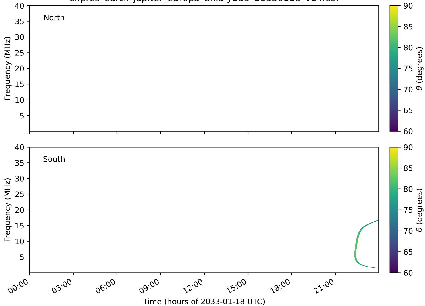
expres_earth_jupiter_europa_txka-y235_20330118_v14.cdf
