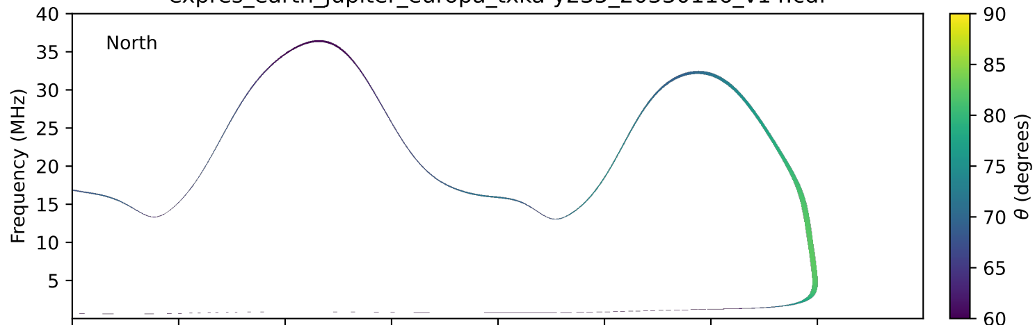
expres_earth_jupiter_europa_txka-y235_20330116_v14.cdf
