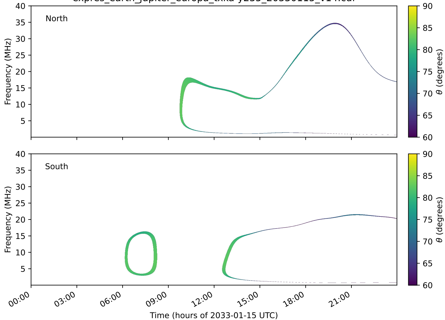
expres_earth_jupiter_europa_txka-y235_20330115_v14.cdf
