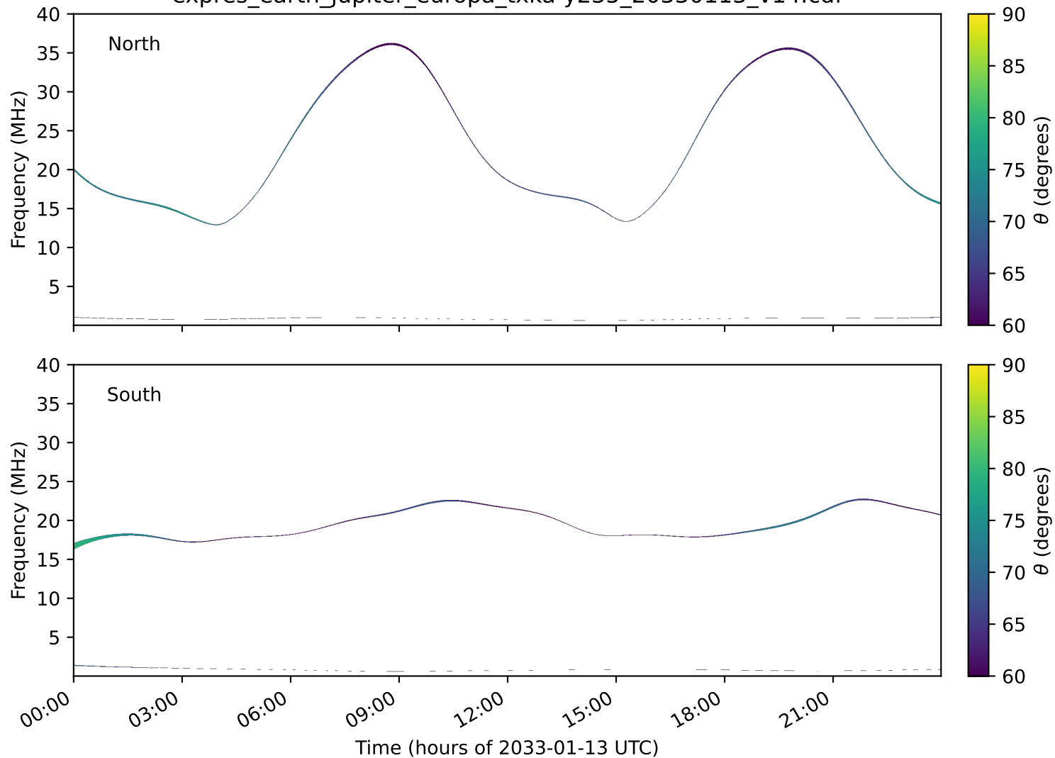
expres_earth_jupiter_europa_txka-y235_20330113_v14.cdf
