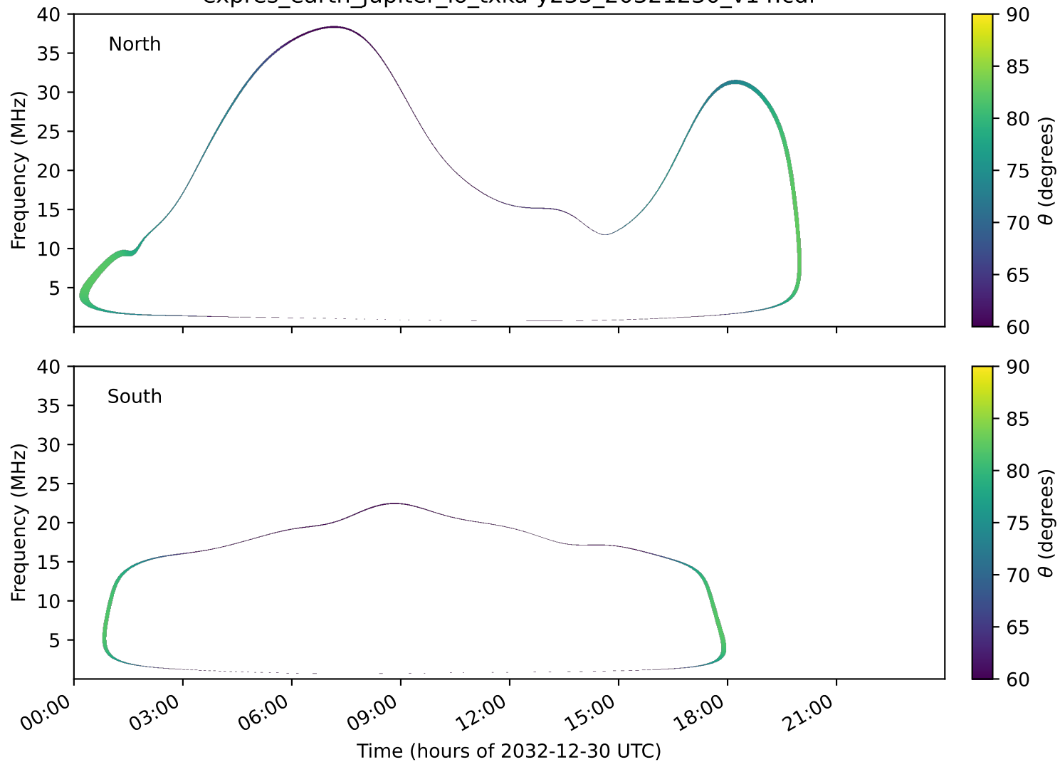
expres_earth_jupiter_io_txka-y235_20321230_v14.cdf
