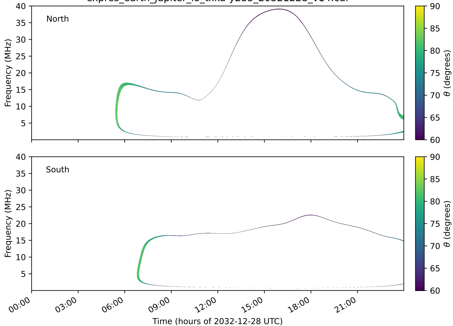
expres_earth_jupiter_io_txka-y235_20321228_v14.cdf
