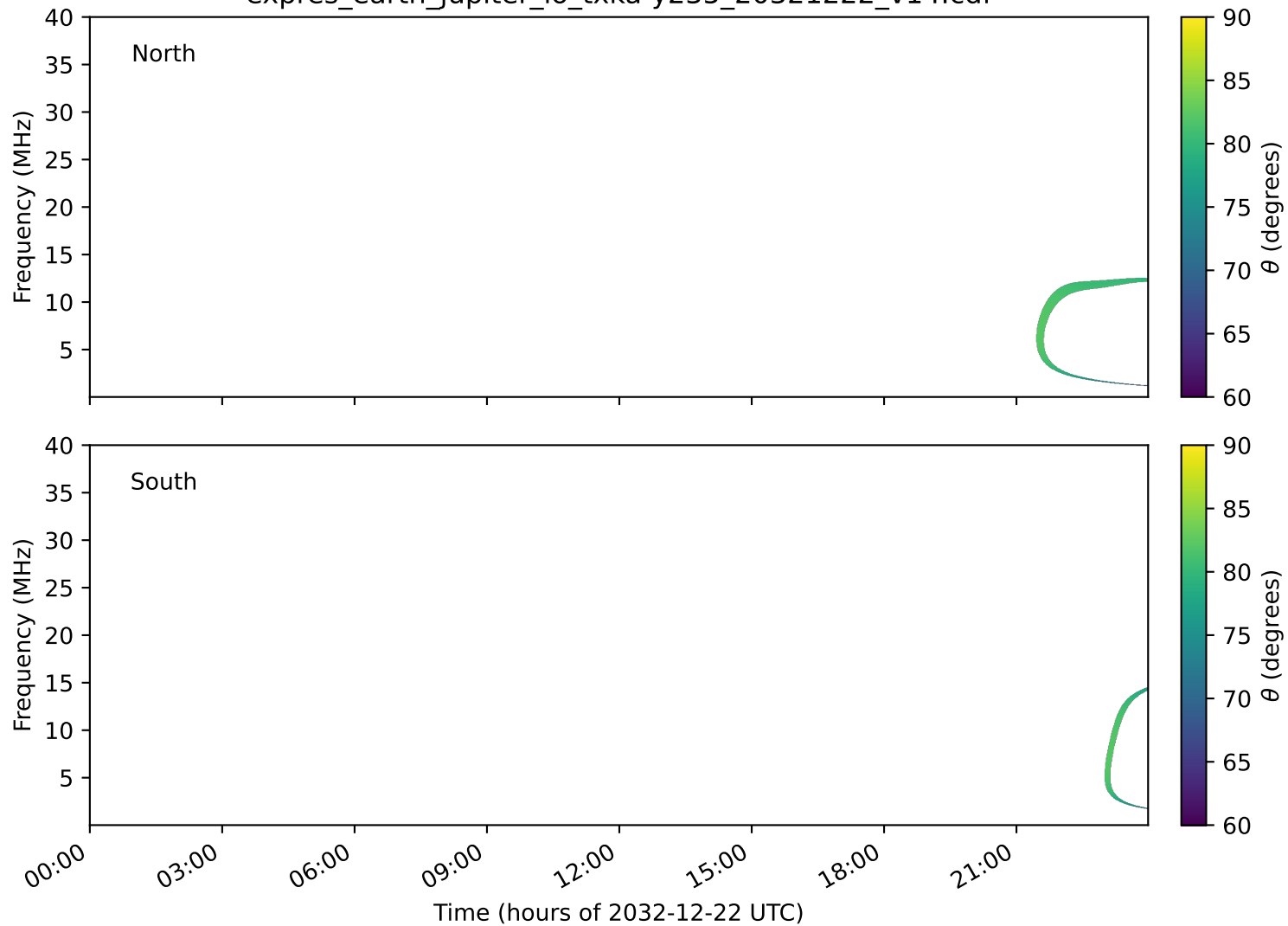
expres_earth_jupiter_io_txka-y235_20321222_v14.cdf
