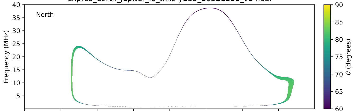
expres_earth_jupiter_io_txka-y235_20321221_v14.cdf
