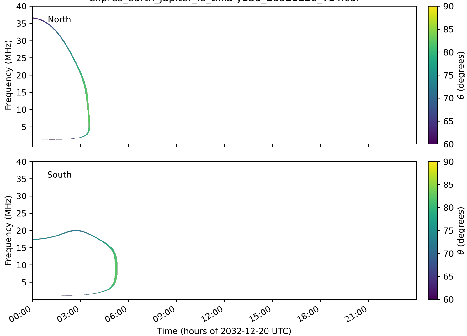
expres_earth_jupiter_io_txka-y235_20321220_v14.cdf
