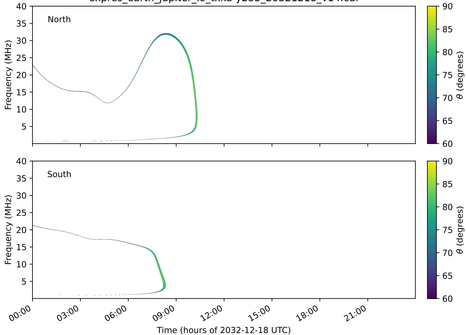
expres_earth_jupiter_io_txka-y235_20321218_v14.cdf
