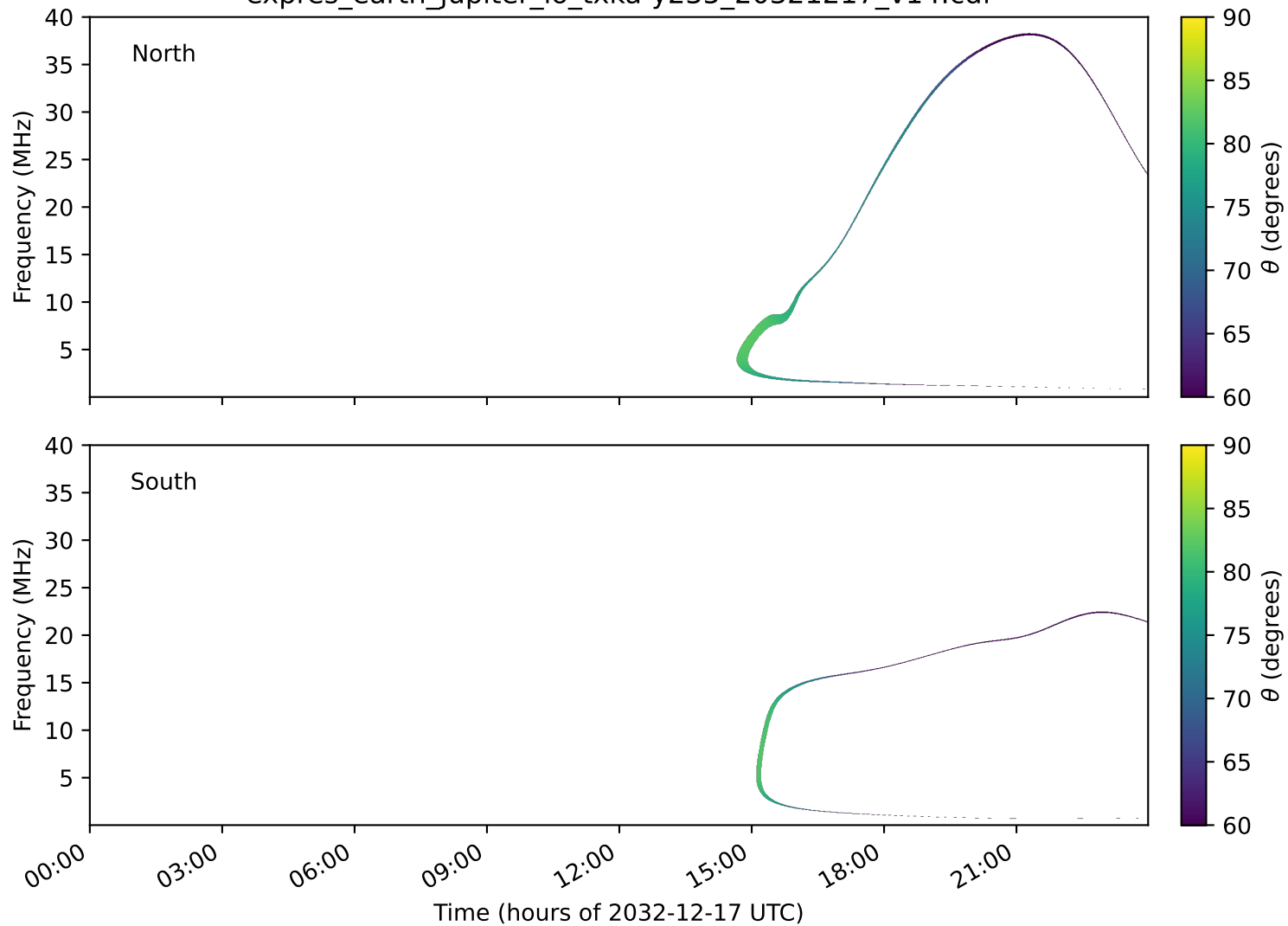
expres_earth_jupiter_io_txka-y235_20321217_v14.cdf
