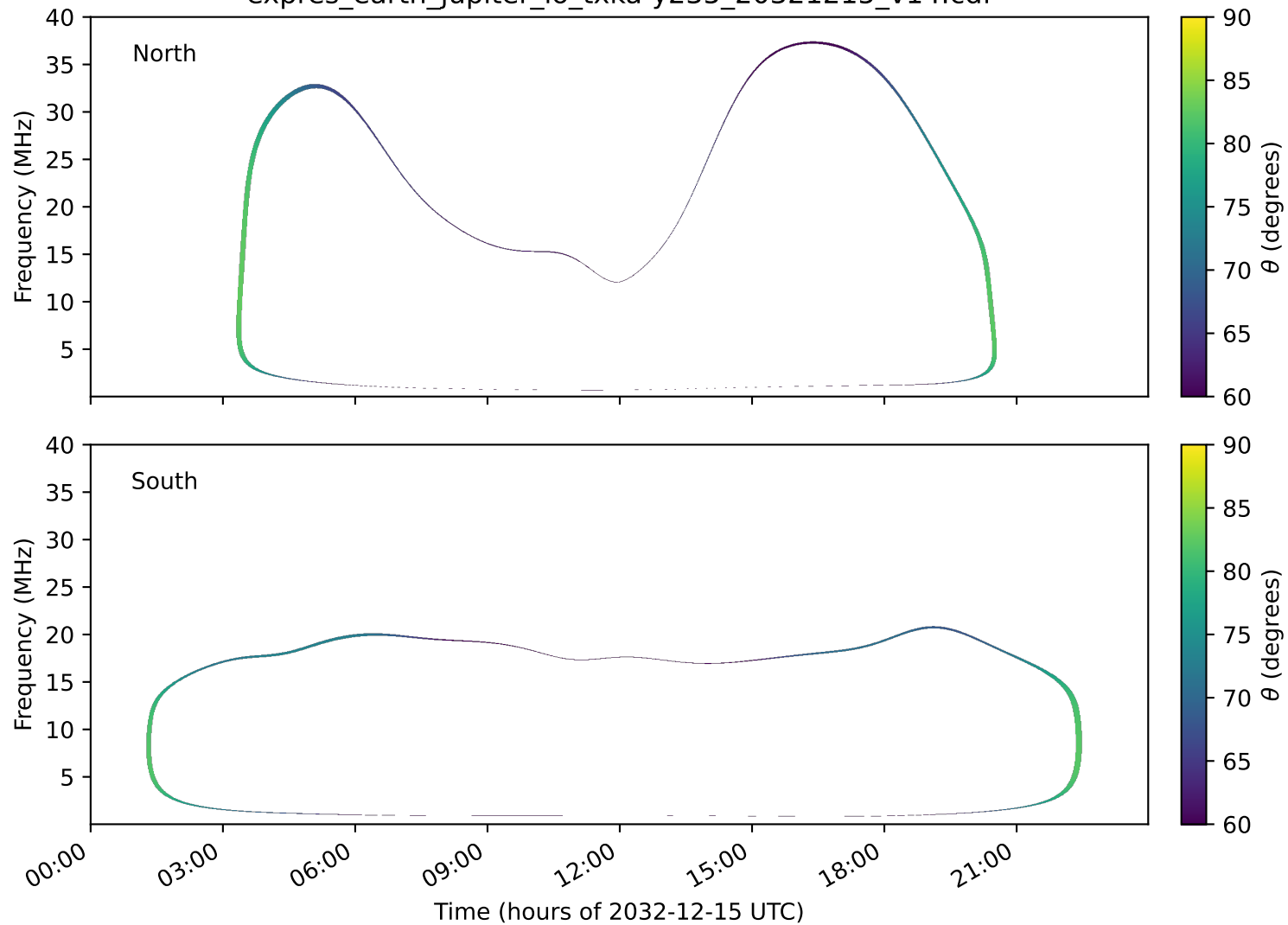
expres_earth_jupiter_io_txka-y235_20321215_v14.cdf
