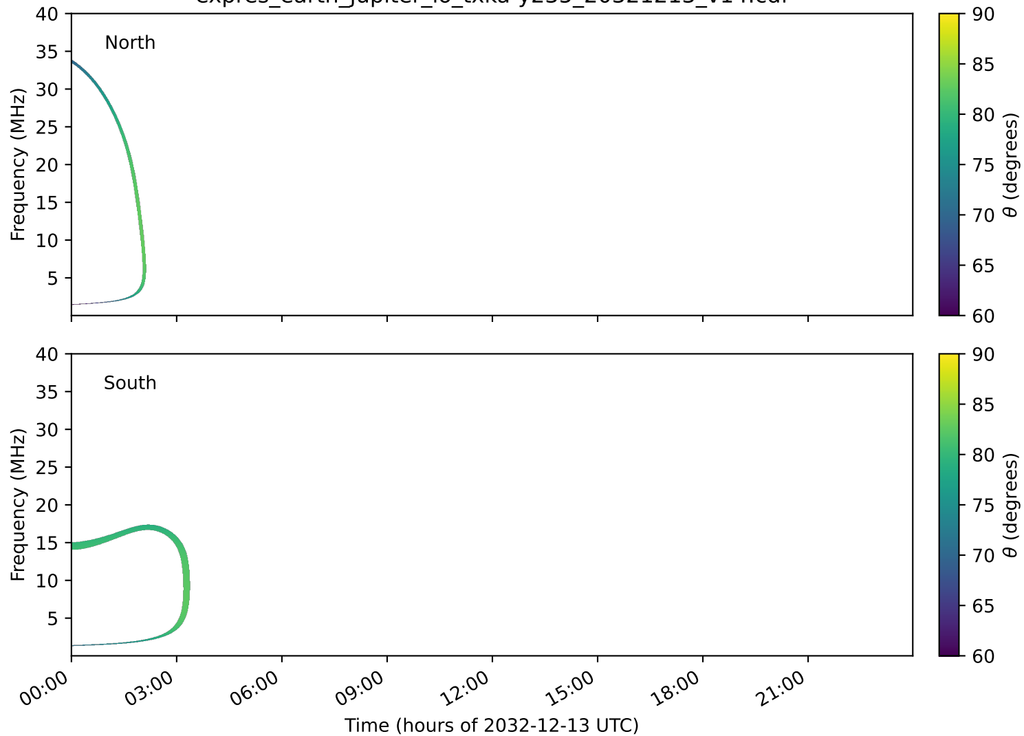
expres_earth_jupiter_io_txka-y235_20321213_v14.cdf
