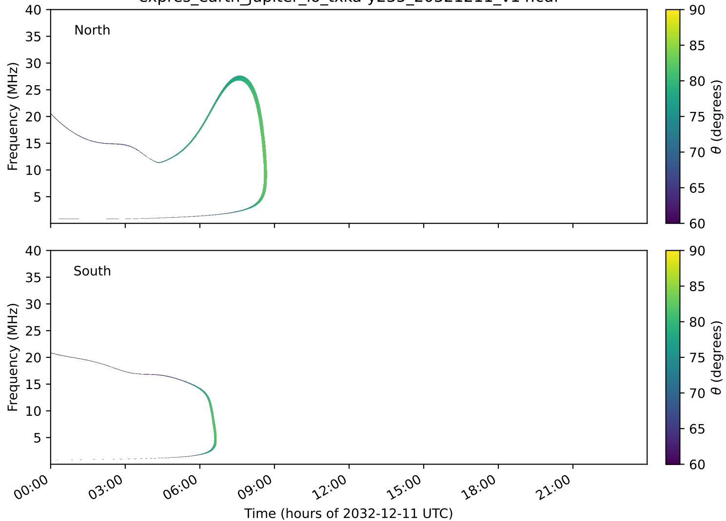
expres_earth_jupiter_io_txka-y235_20321211_v14.cdf
