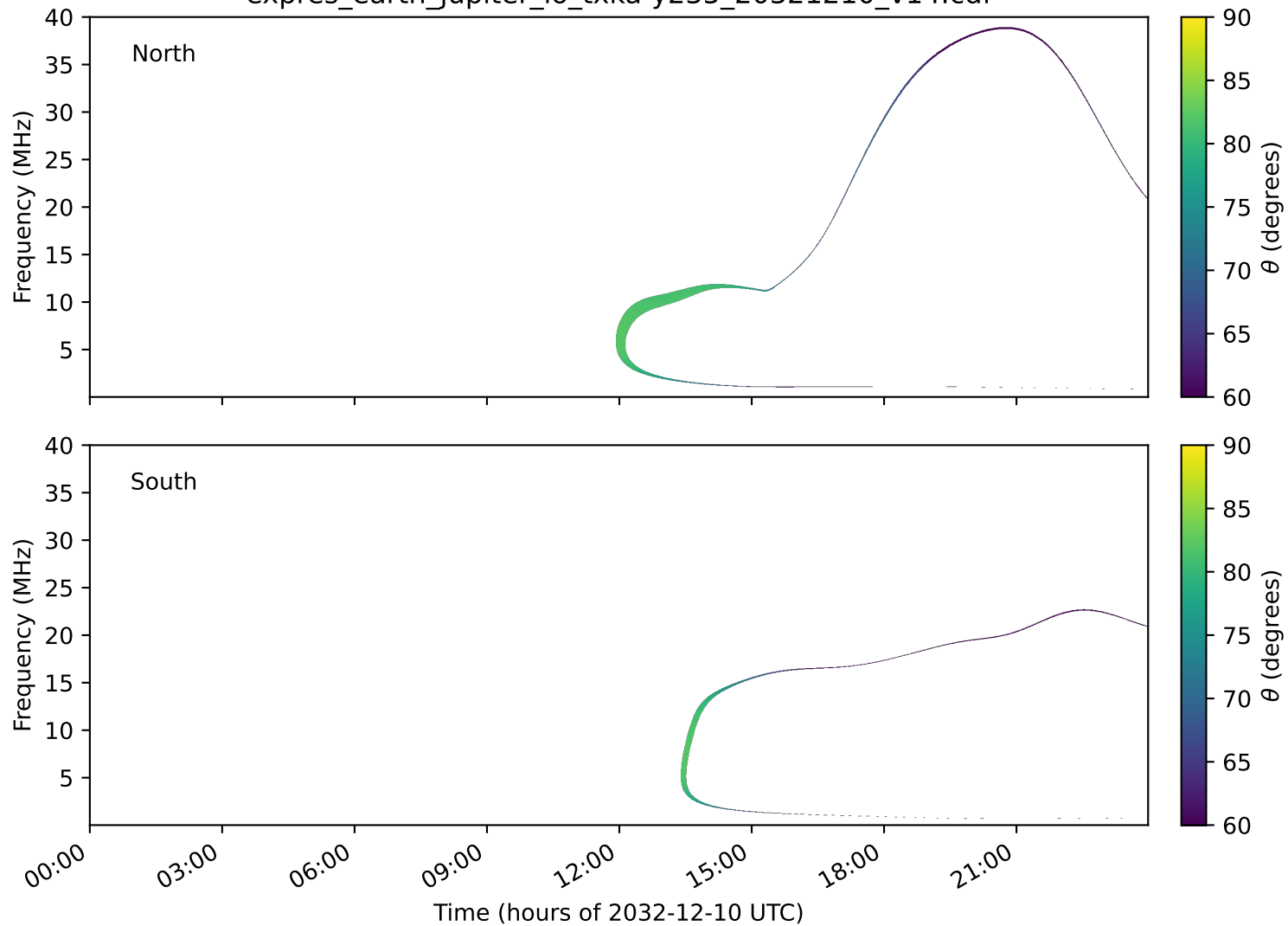
expres_earth_jupiter_io_txka-y235_20321210_v14.cdf
