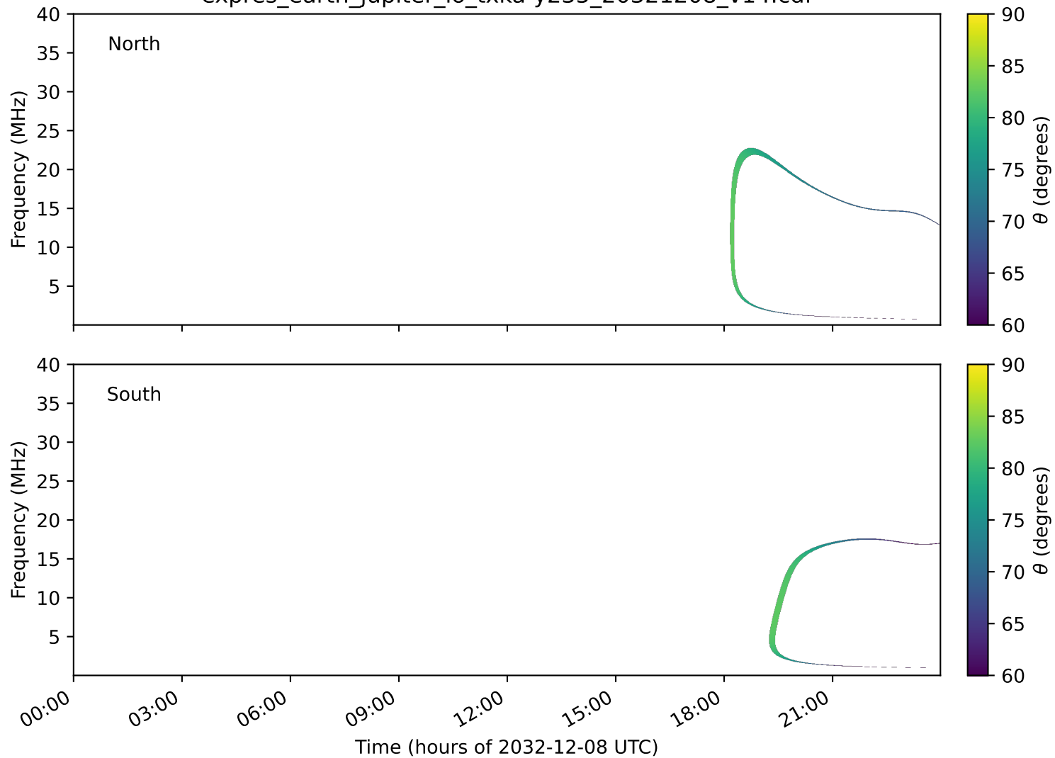
expres_earth_jupiter_io_txka-y235_20321208_v14.cdf
