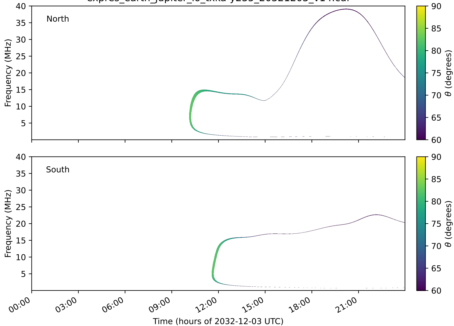
expres_earth_jupiter_io_txka-y235_20321203_v14.cdf
