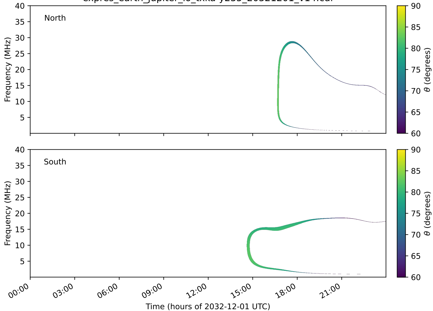
expres_earth_jupiter_io_txka-y235_20321201_v14.cdf
