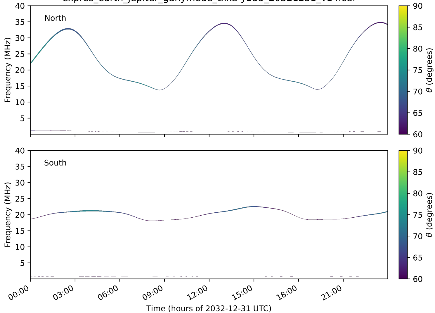
expres_earth_jupiter_ganymede_txka-y235_20321231_v14.cdf
