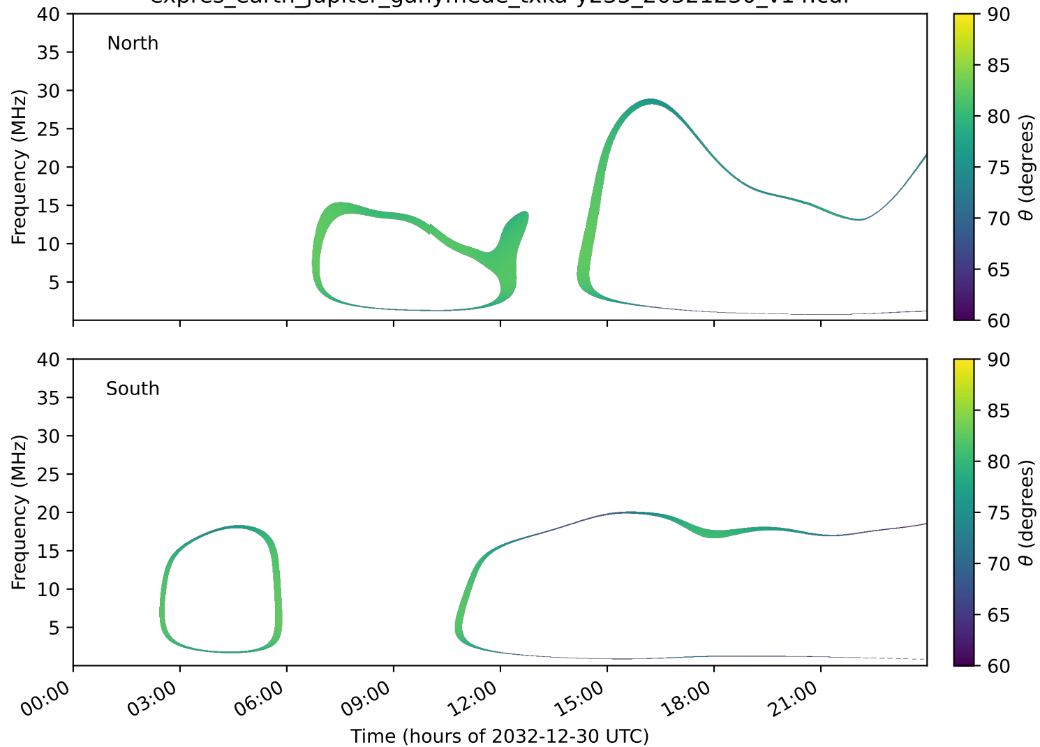
expres_earth_jupiter_ganymede_txka-y235_20321230_v14.cdf
