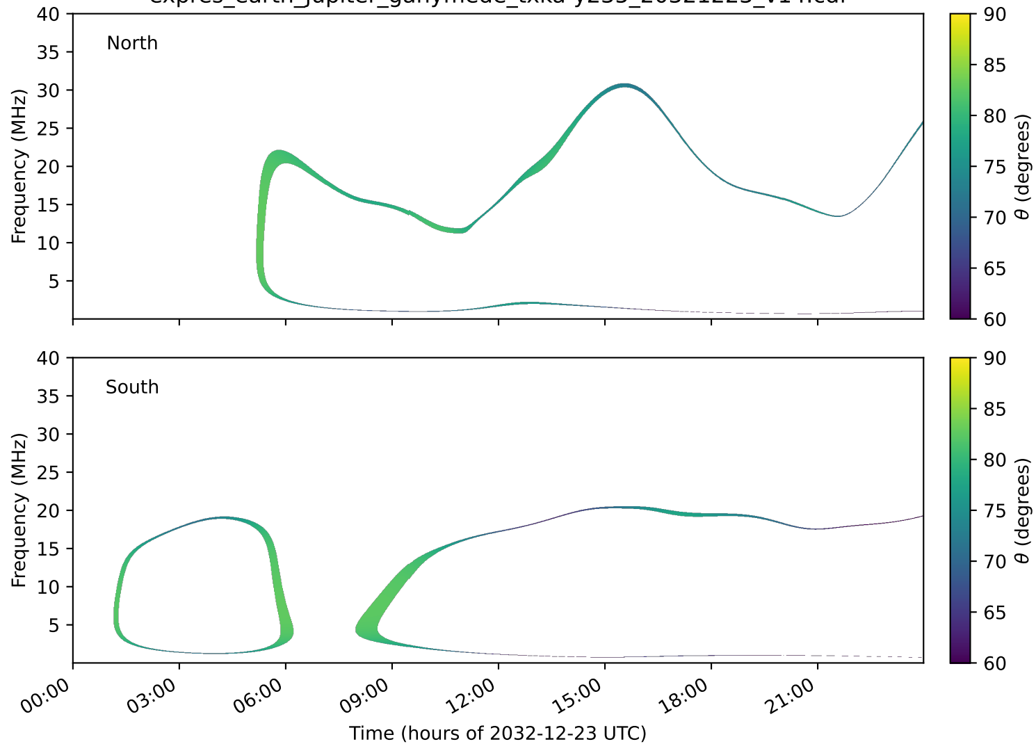
expres_earth_jupiter_ganymede_txka-y235_20321223_v14.cdf
