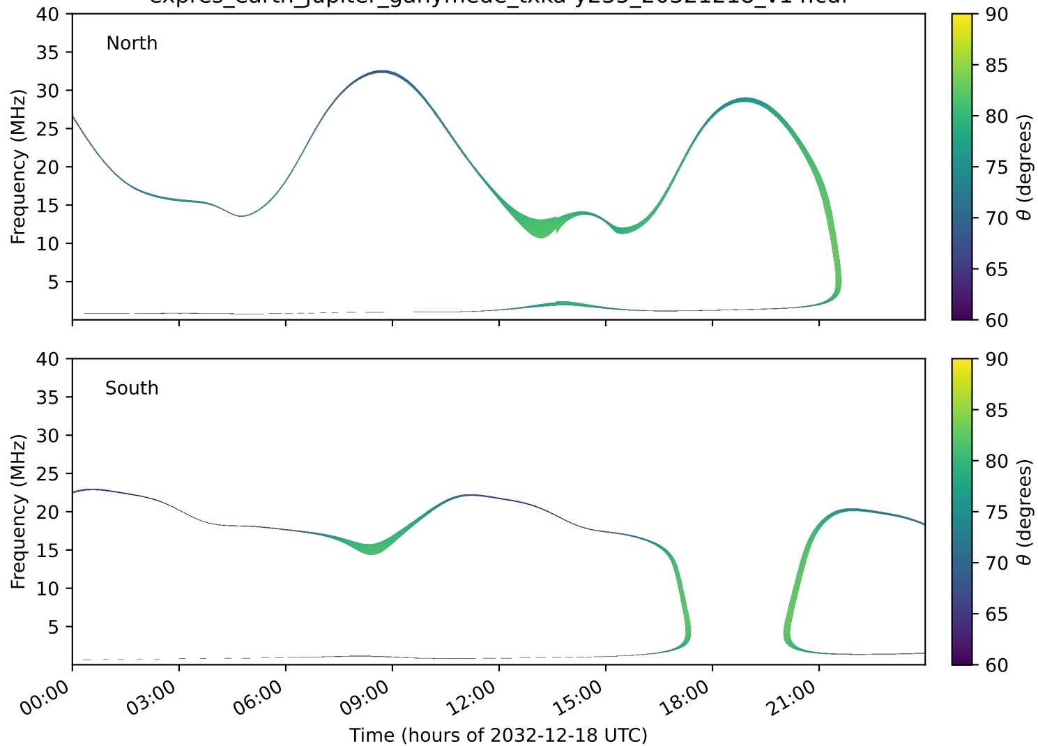
expres_earth_jupiter_ganymede_txka-y235_20321218_v14.cdf
