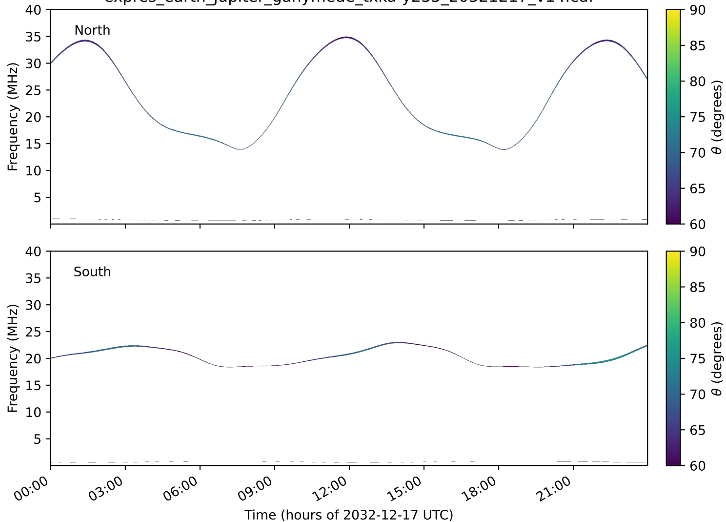
expres_earth_jupiter_ganymede_txka-y235_20321217_v14.cdf
