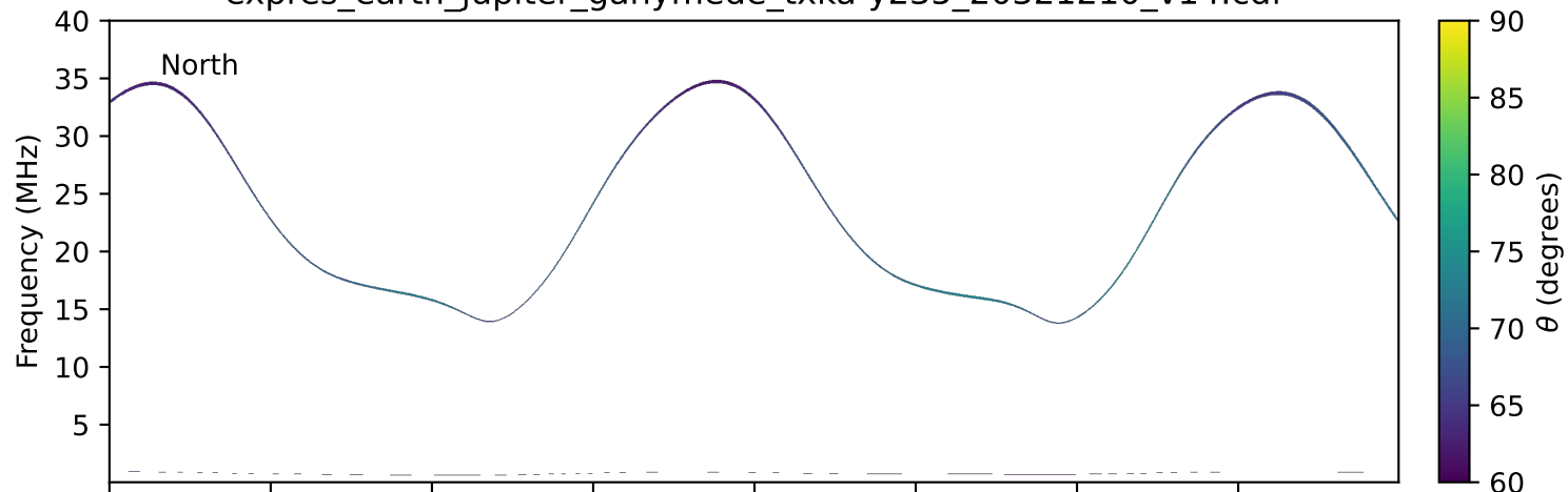
expres_earth_jupiter_ganymede_txka-y235_20321210_v14.cdf
