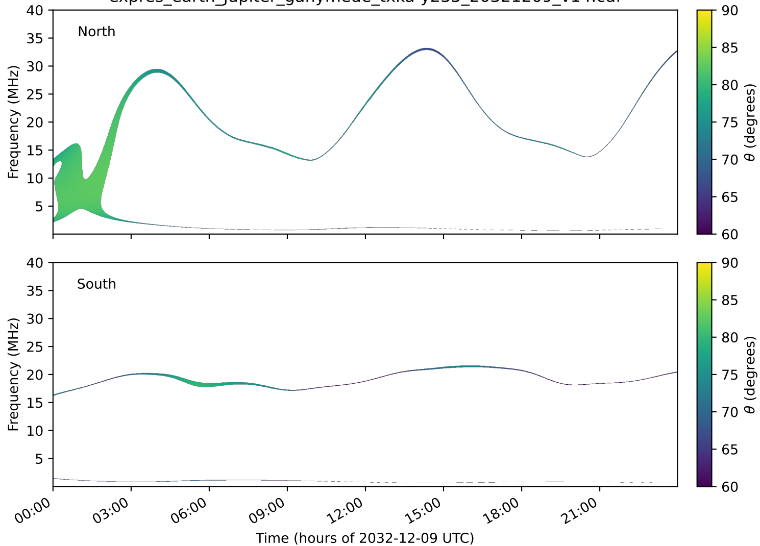
expres_earth_jupiter_ganymede_txka-y235_20321209_v14.cdf
