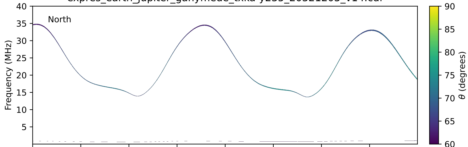
expres_earth_jupiter_ganymede_txka-y235_20321203_v14.cdf
