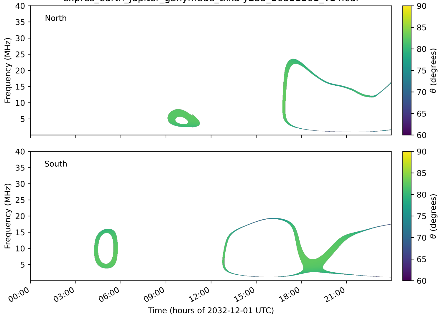
expres_earth_jupiter_ganymede_txka-y235_20321201_v14.cdf
