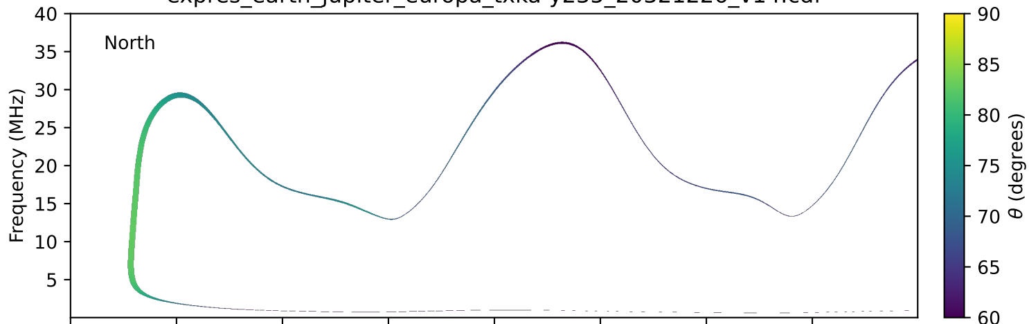
expres_earth_jupiter_europa_txka-y235_20321226_v14.cdf
