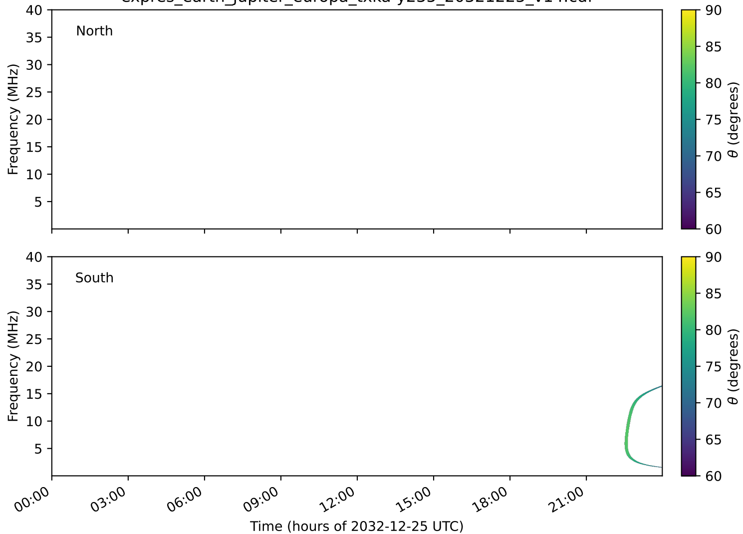
expres_earth_jupiter_europa_txka-y235_20321225_v14.cdf
