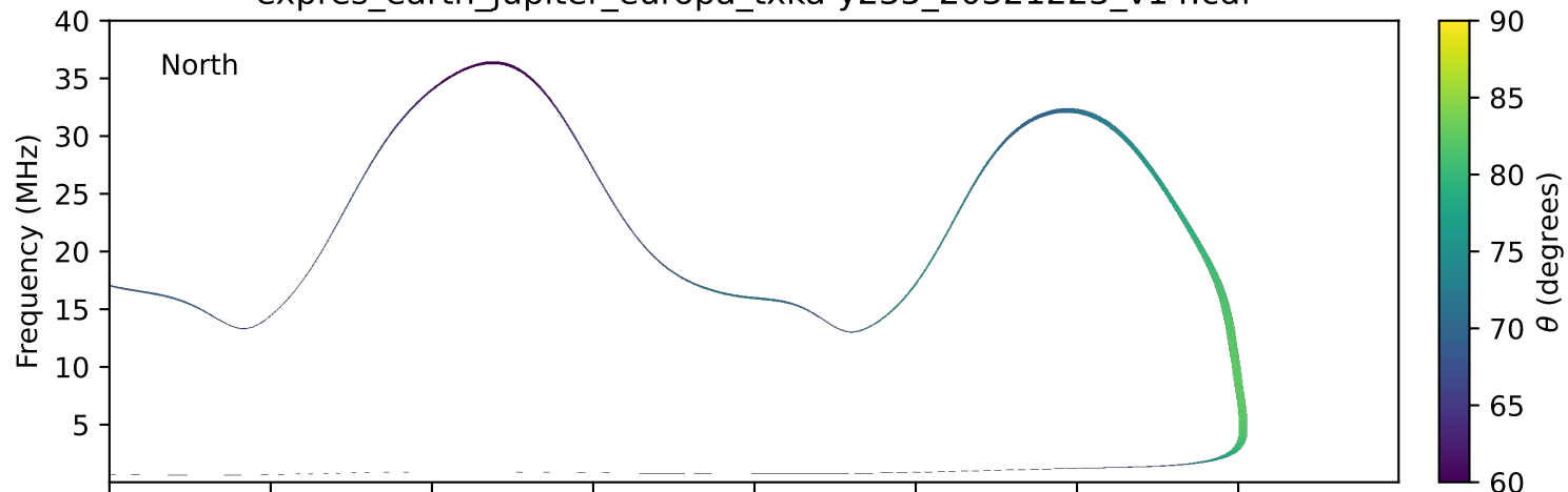
expres_earth_jupiter_europa_txka-y235_20321223_v14.cdf
