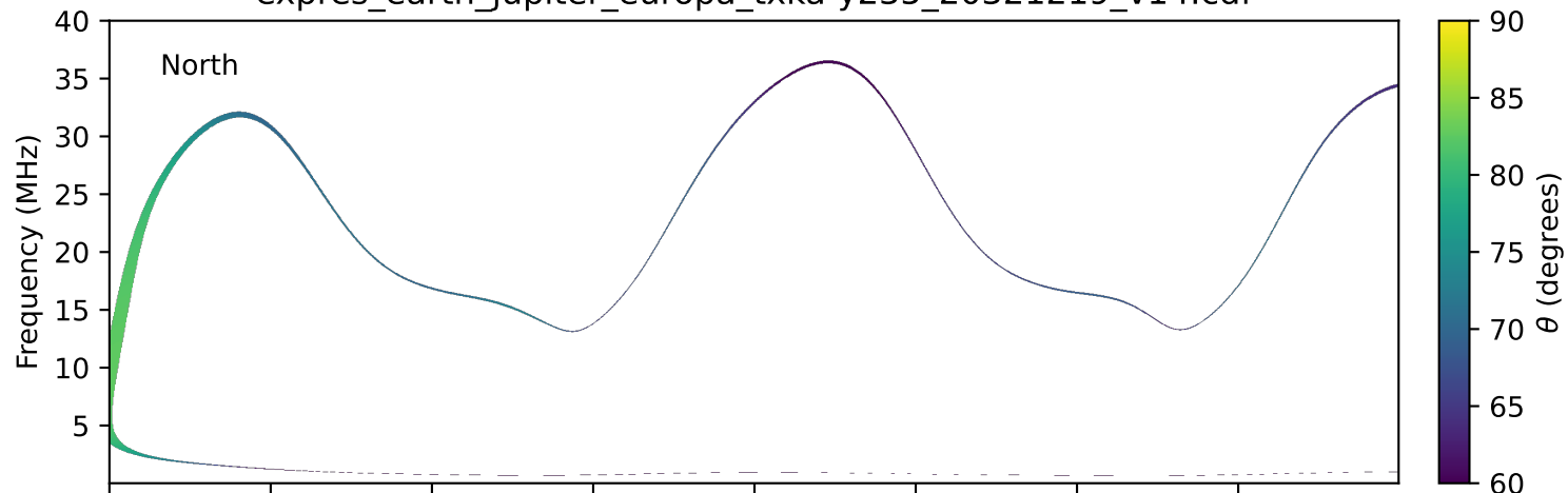
expres_earth_jupiter_europa_txka-y235_20321219_v14.cdf
