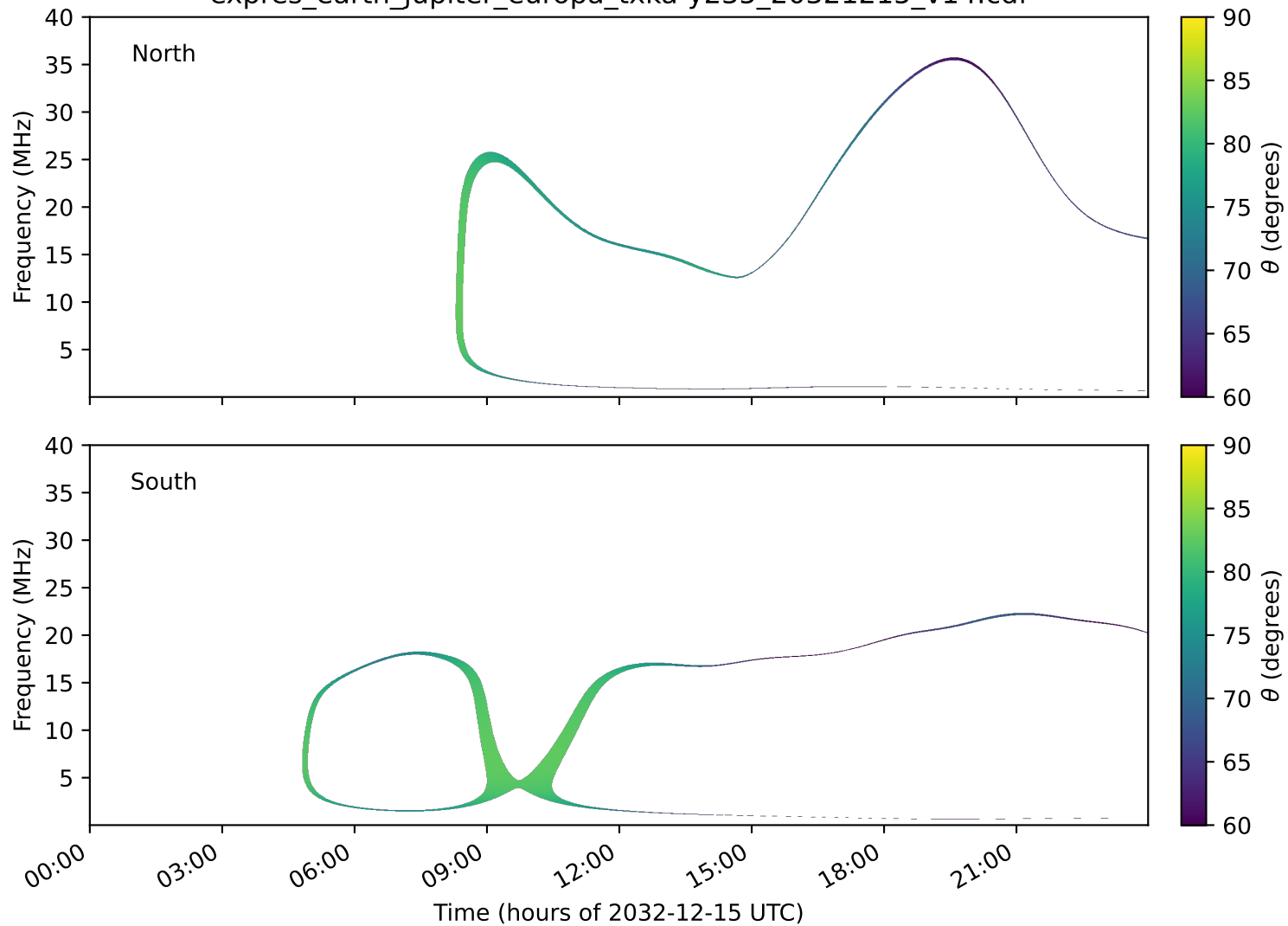
expres_earth_jupiter_europa_txka-y235_20321215_v14.cdf
