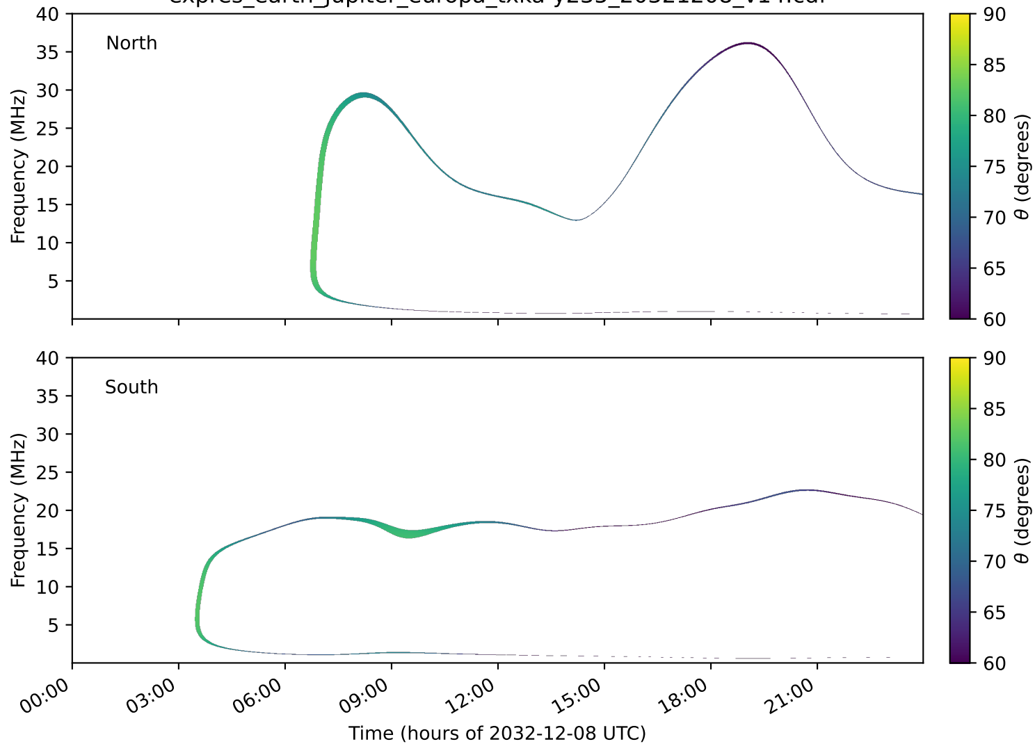
expres_earth_jupiter_europa_txka-y235_20321208_v14.cdf
