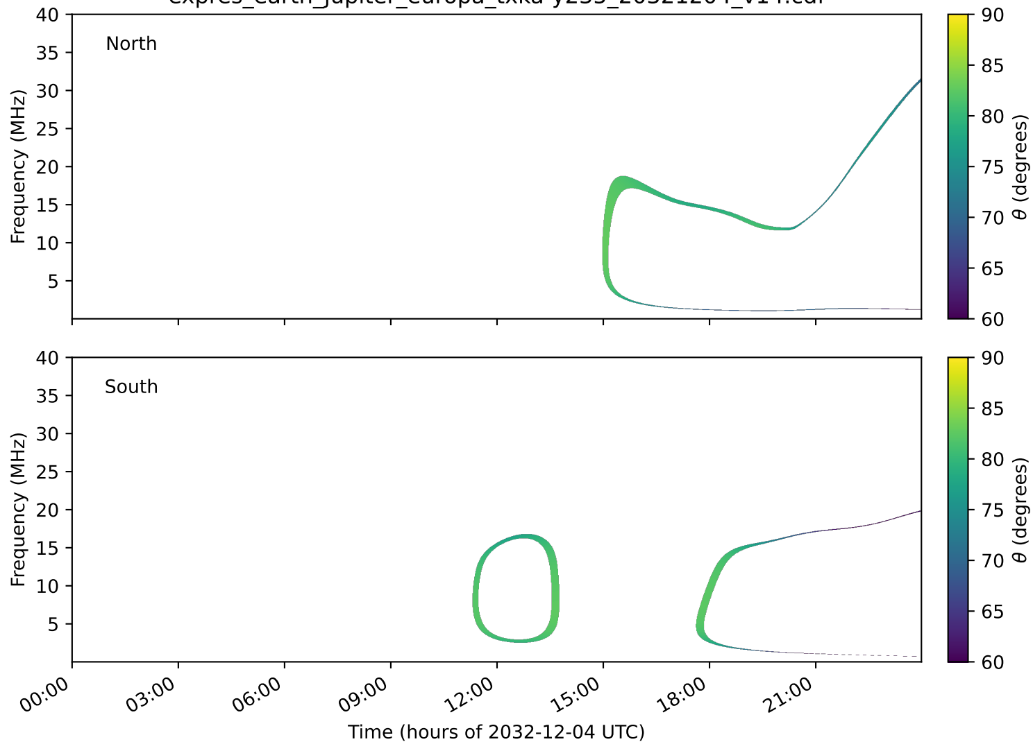
expres_earth_jupiter_europa_txka-y235_20321204_v14.cdf
