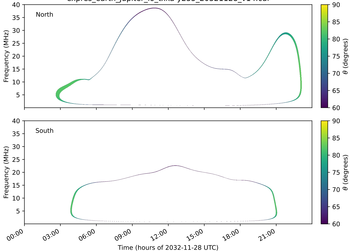
expres_earth_jupiter_io_txka-y235_20321128_v14.cdf
