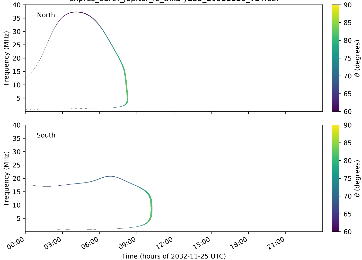
expres_earth_jupiter_io_txka-y235_20321125_v14.cdf
