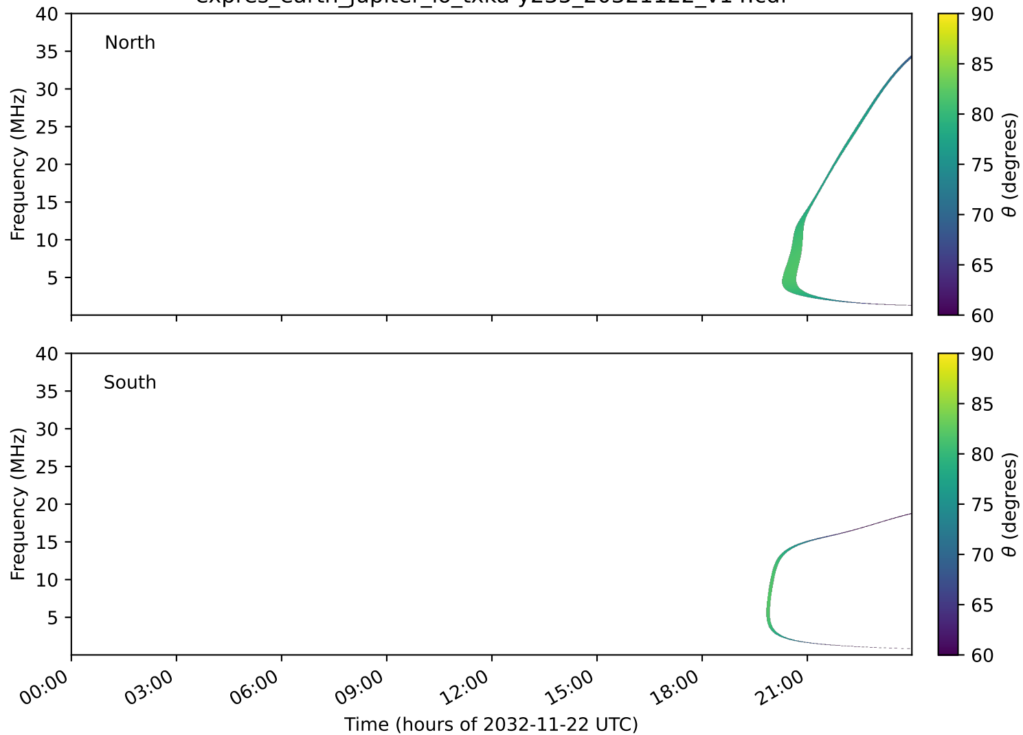
expres_earth_jupiter_io_txka-y235_20321122_v14.cdf
