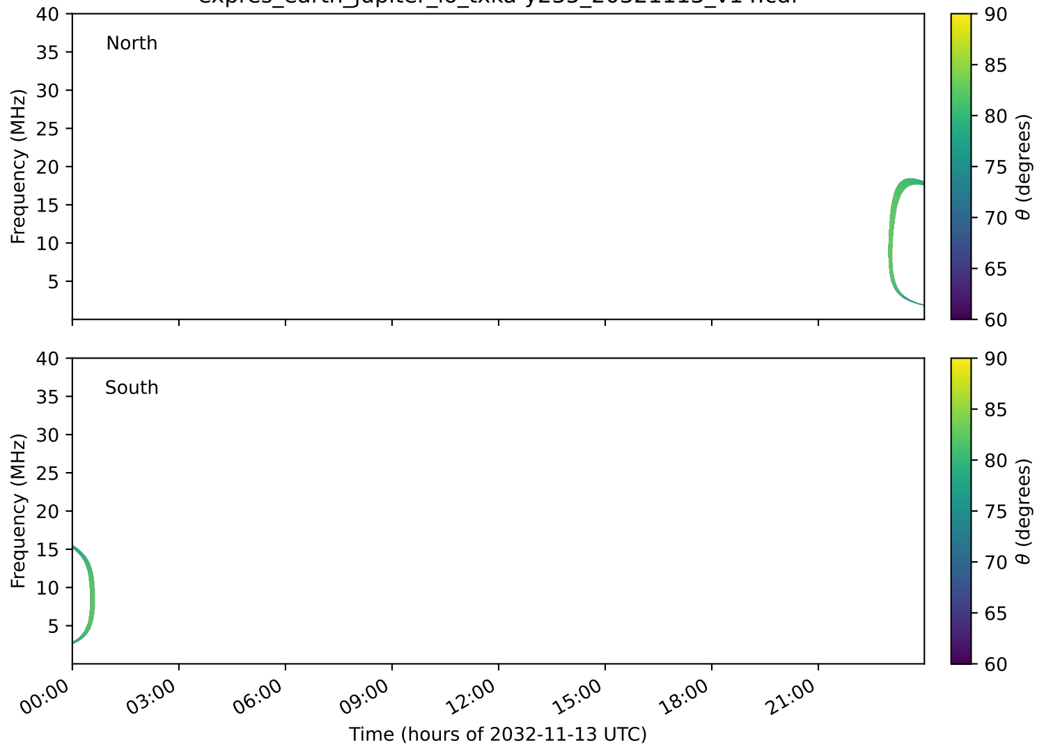
expres_earth_jupiter_io_txka-y235_20321113_v14.cdf
