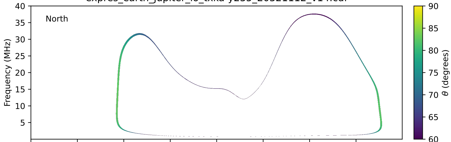
expres_earth_jupiter_io_txka-y235_20321112_v14.cdf
