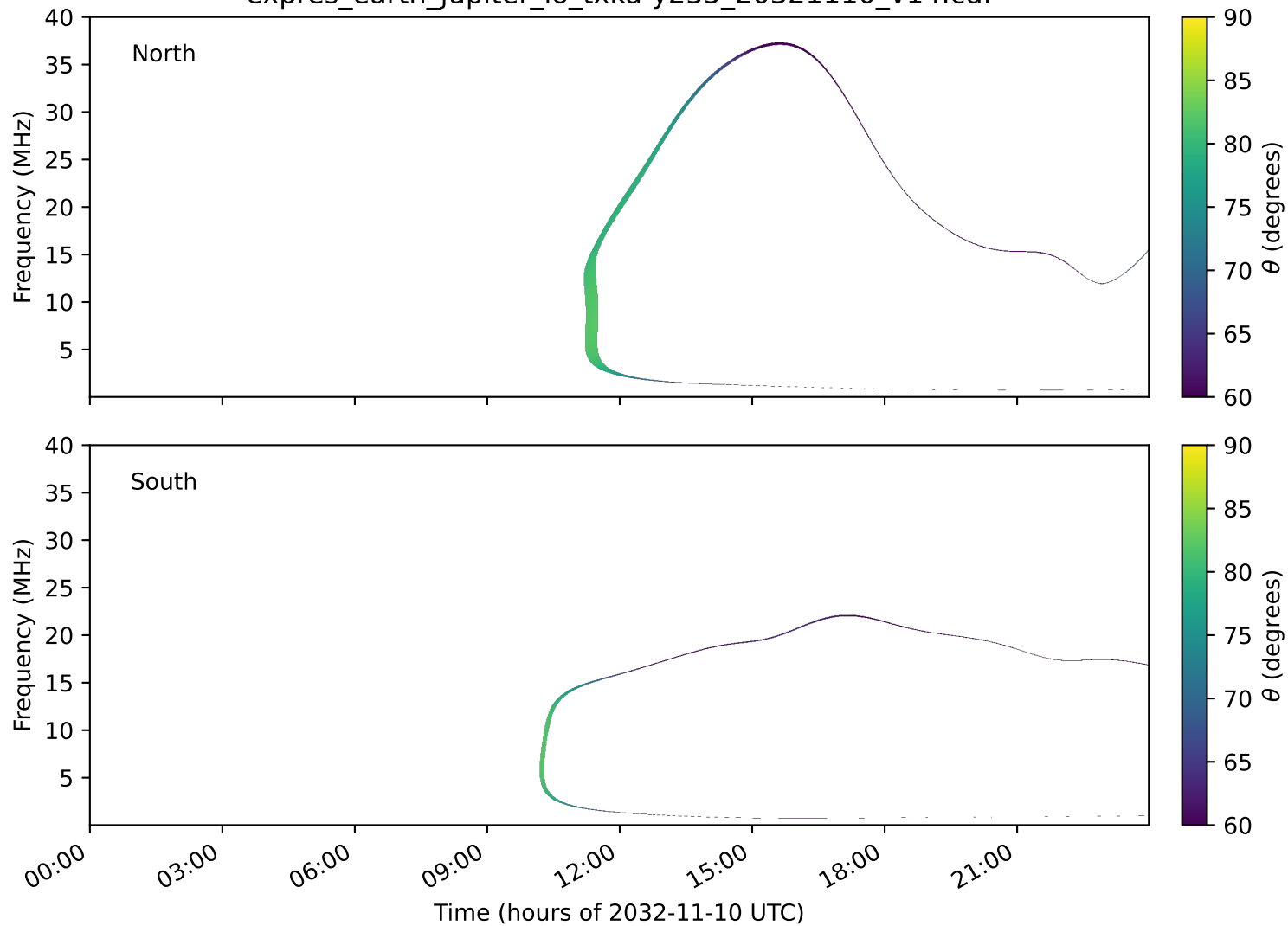
expres_earth_jupiter_io_txka-y235_20321110_v14.cdf
