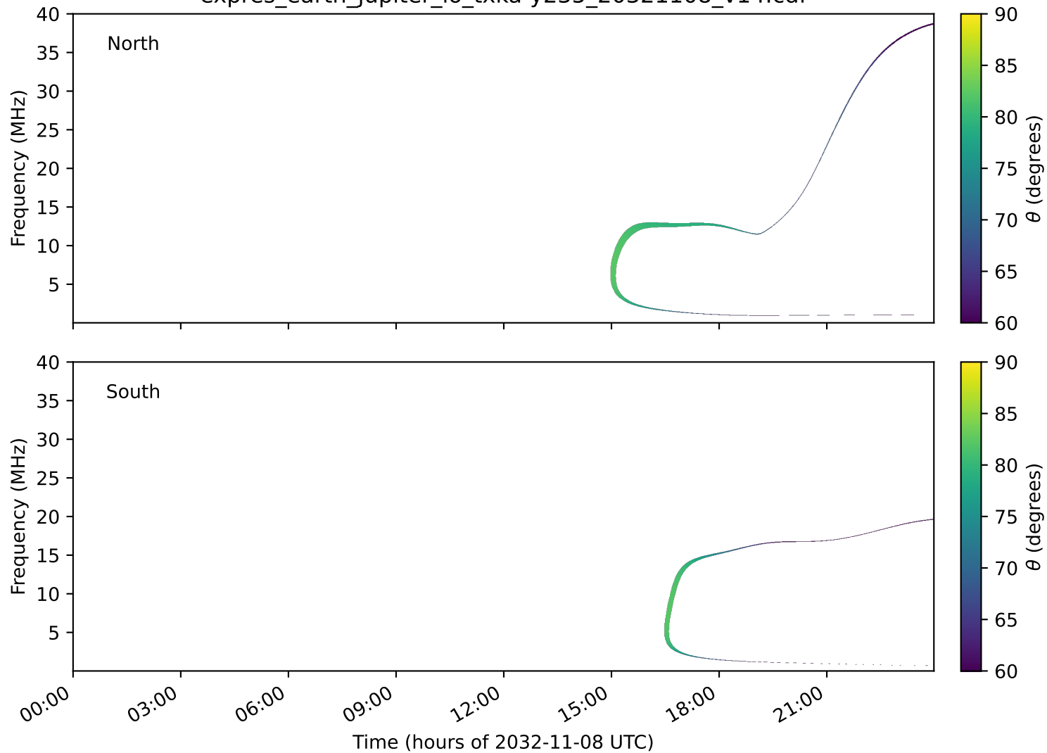
expres_earth_jupiter_io_txka-y235_20321108_v14.cdf
