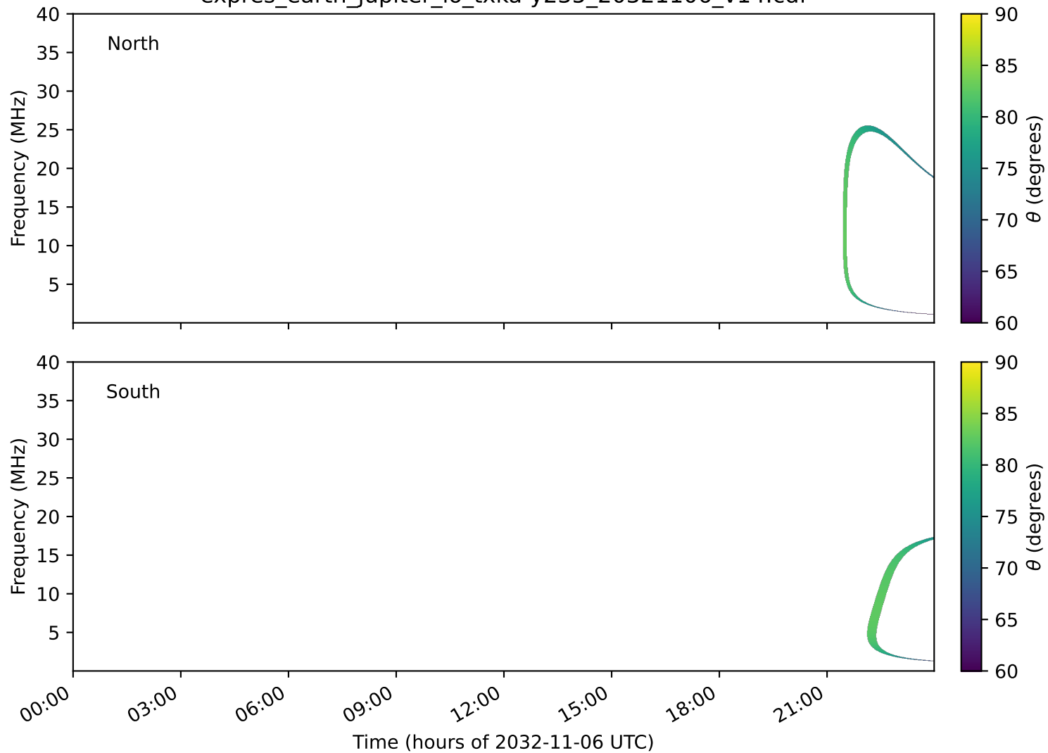
expres_earth_jupiter_io_txka-y235_20321106_v14.cdf
