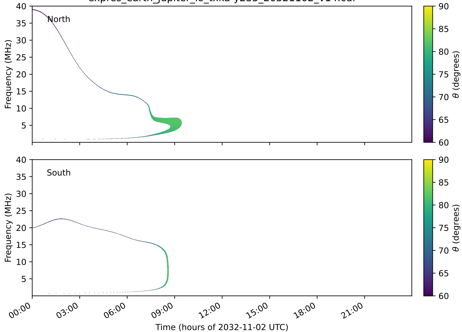
expres_earth_jupiter_io_txka-y235_20321102_v14.cdf
