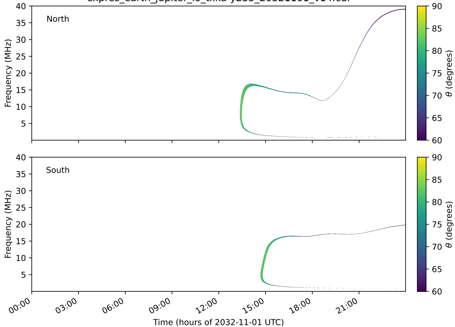
expres_earth_jupiter_io_txka-y235_20321101_v14.cdf
